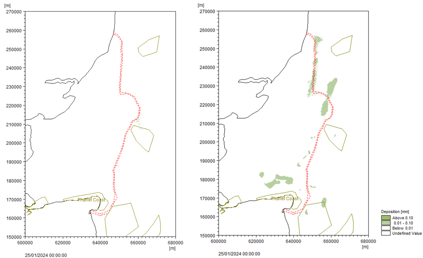
Plate 4.1.43 Depth of deposition with jetting installation for mud (left) and fine sand (right) at end of 14-day period.
