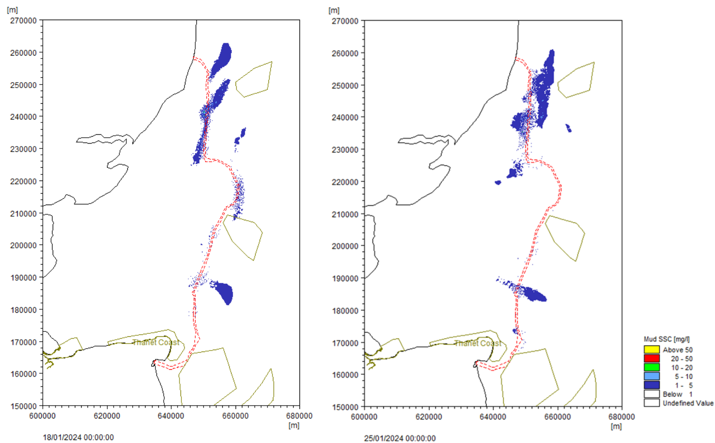
Plate 4.1.39 Mud SSC levels for jetting installation commencing on spring tides with output at +7 days (left) and +14 days (right) after start of activity
