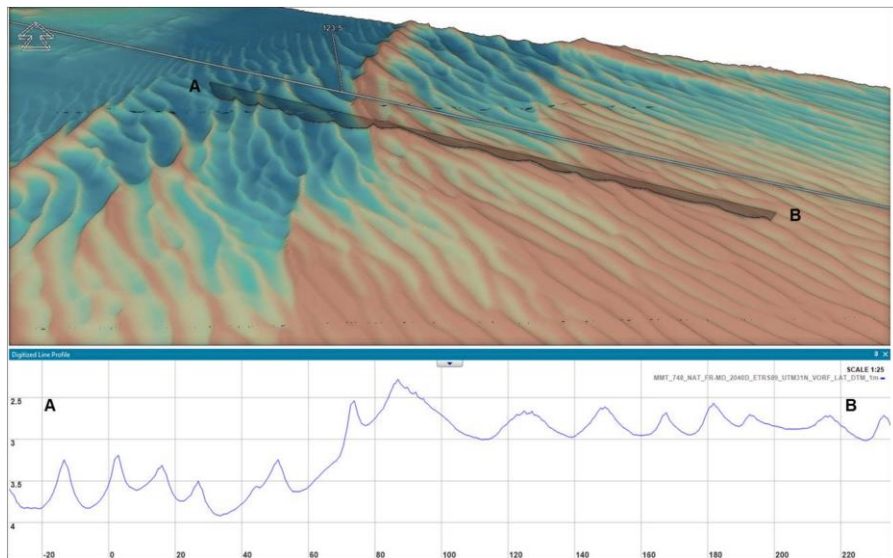
Plate 4.1.34 Slopes along the route associated with lee slopes of a mega ripple area at KP 117 (MMT, 2022).
