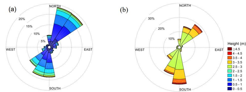
Plate 1.1.2 From Atkinson and Esteves (Atkinson & Esteves, 2019) – West Gabbard buoy wave roses for (a) all waves and (b) waves of Hs > 2.5 m, showing the percentage of waves of different heights (Hs) that approach from different directions in the period June 2006 to March 2018 (168685 records, 98% data coverage).
