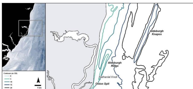
Plate 1.7.1 Thames Estuary bedforms near the Suffolk Coastline, including the Aldeburgh Napes and Aldeburgh Ridge (Burningham & French, 2008).
