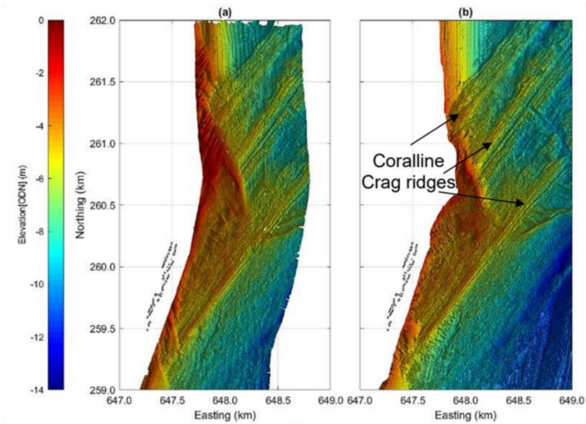
Plate 4.1.5 Bathymetry obtained from two multibeam surveys undertaken by (A) the EA in June 2014 and (B) the Maritime Coastal Authority in January 2017. From (Royal Haskoning DHV, 2019).
