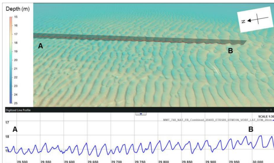
Plate 4.1.31 Example of the sand waves near KP 22 - KP 26. Maximum height 1 m. The red line in the image does not correspond to updated Offshore Scheme route (MMT, 2022).
