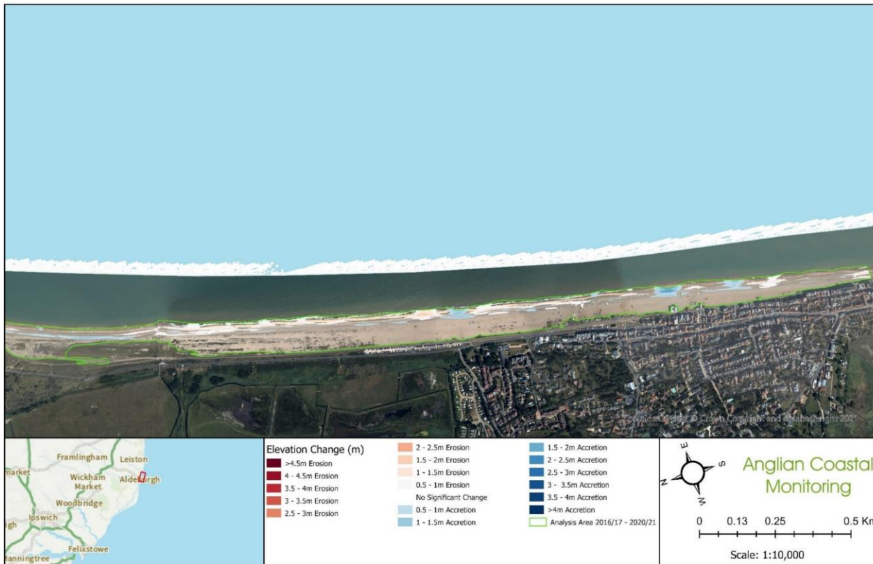
Plate 4.1.14 The difference in elevation from the LiDAR survey in 2016 and the most recent survey in 2021 for the Aldeburgh monitoring cell (Anglian Regional Coastal Monitoring Programme, 2022).
