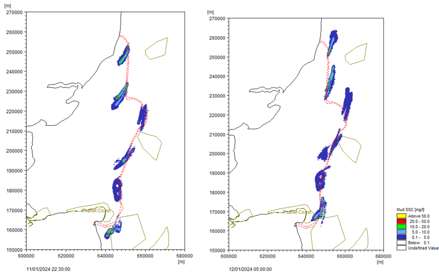
Plate 4-1.38 Mud SSC levels for jetting installation commencing on spring tides with output on flood (left) and ebb (right) tide after first 24 hours of activity
