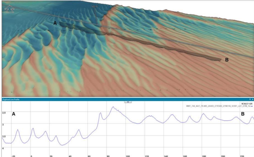
Plate 4.1.27 Bedforms along the route associated with lee slopes of a mega ripple area at KP 123.475 (MMT, 2022)
