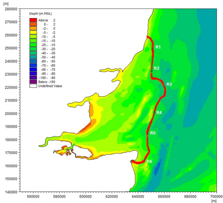
Plate 4.1.37 Hydrodynamic model bathymetry showing the Offshore Scheme Boundary (red line) and 6 sediment release locations
