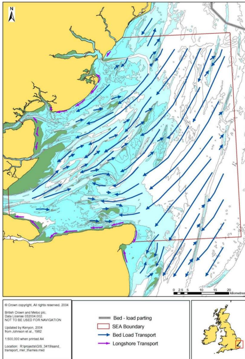
Plate 4.1.22 Map of net sand transport paths in the Outer Thames Estuary (Kenyon & Cooper, 2005).
