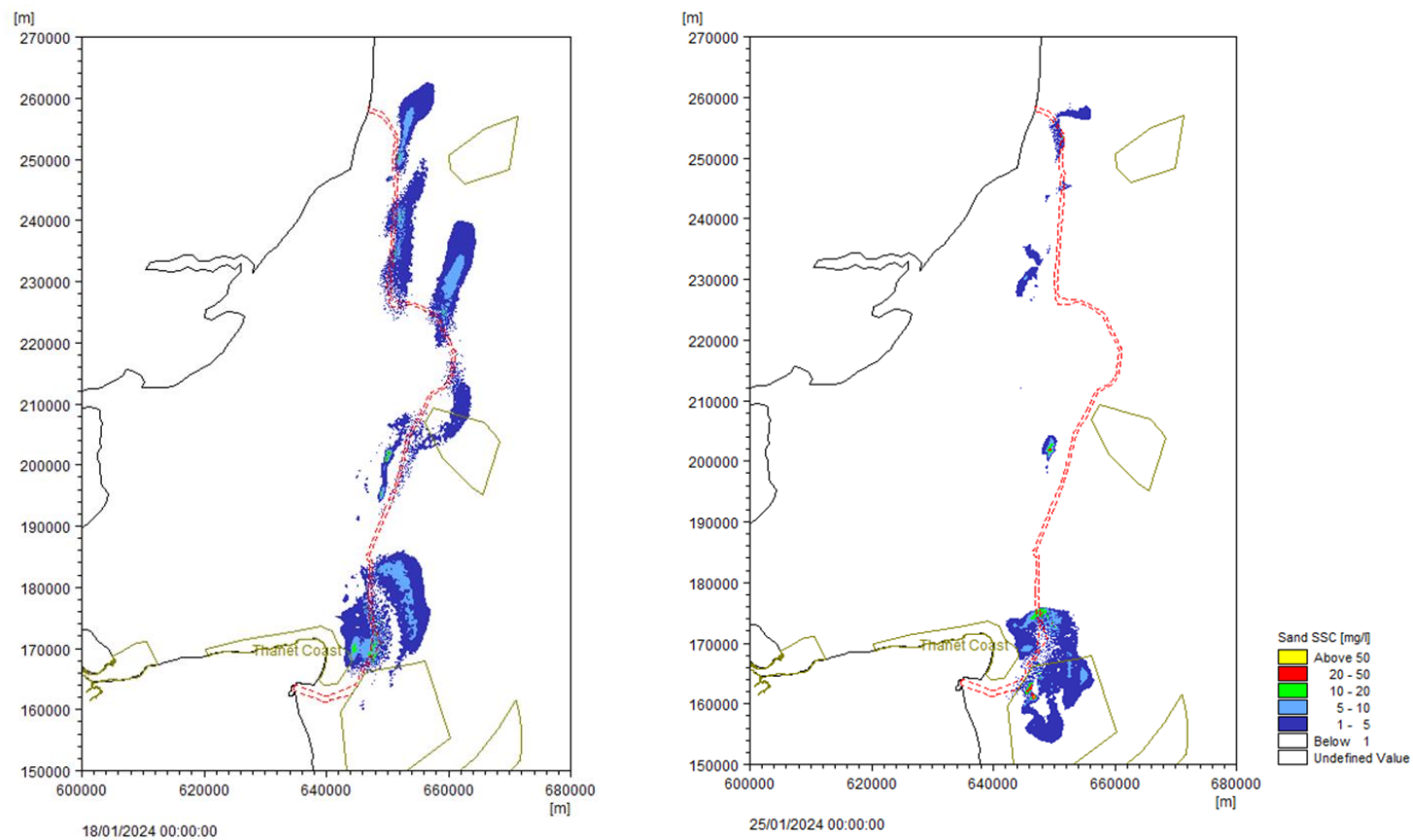
Plate 4.1.41 Sand SSC levels for jetting installation commencing on spring tides with output at +7 days (left) and +14 days (right) after start of activity
