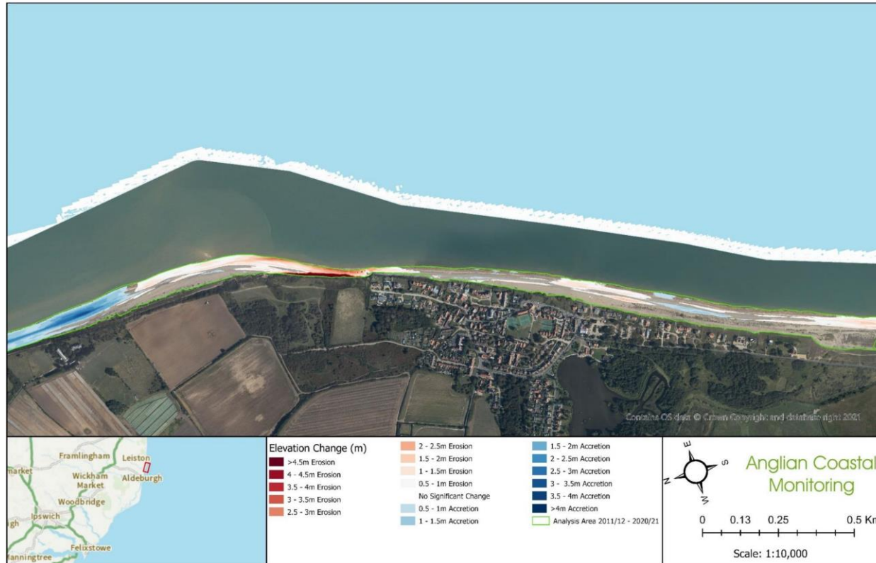
Plate 4.1.10 The difference in elevation from the first LiDAR survey in 2011 and the most recent survey in 2021 for the Thorpeness monitoring cell (Anglian Regional Coastal Monitoring Programme, 2022).
