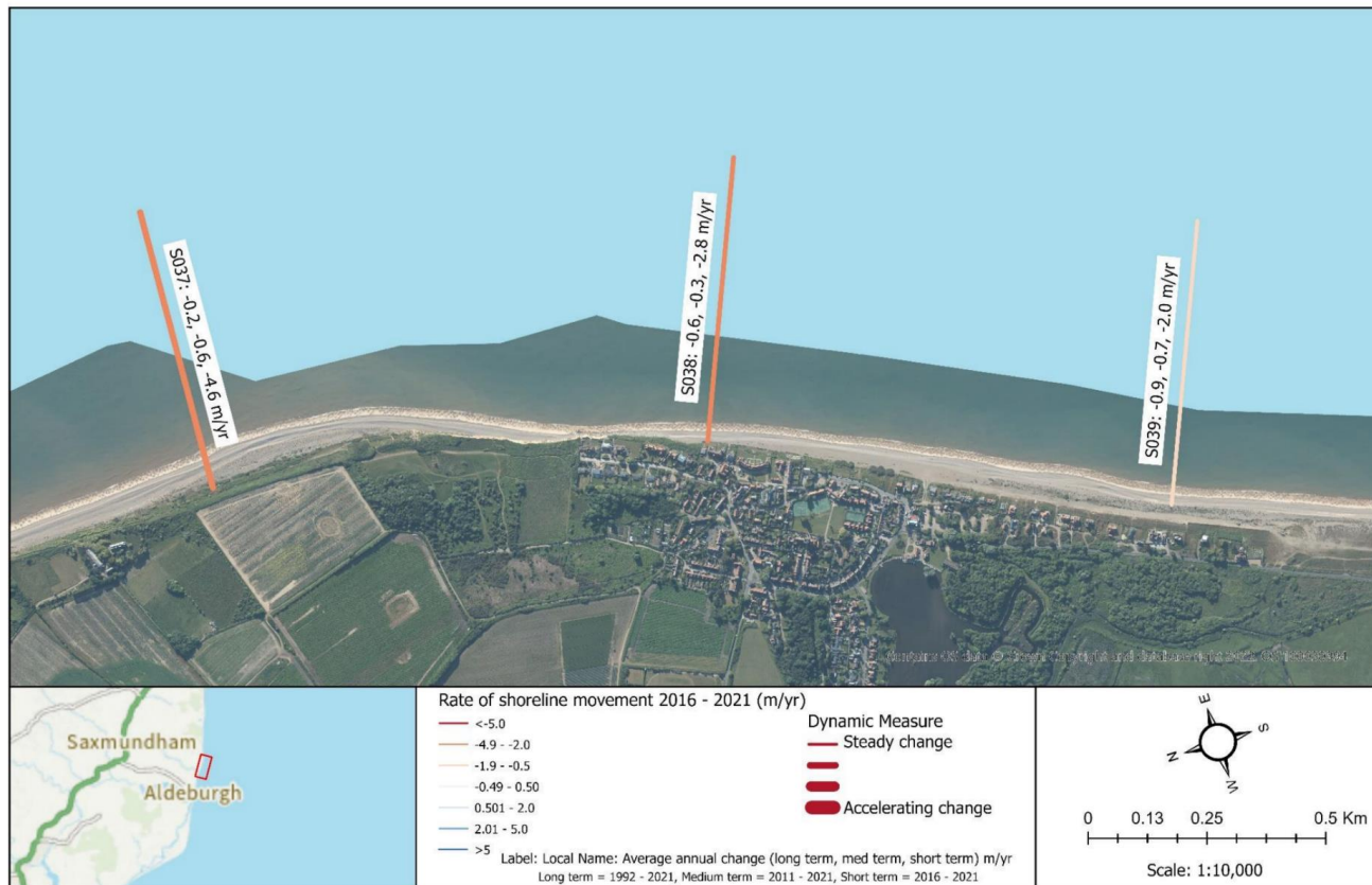
Plate 4.1.11 Rates of Shoreline Movement (at Mean Sea Level) for the Thorpeness monitoring cell (Anglian Regional Coastal Monitoring Programme, 2022).
