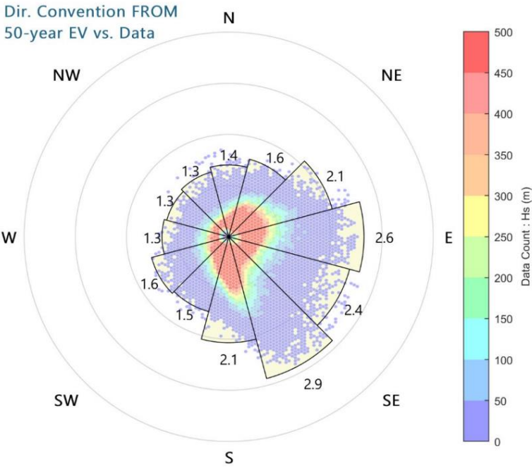
Plate 4.1.3 Wave rose of extreme wave heights at 1:50 return period for KP3, showing the amount of wave height data per sector and in black the extreme wave height per direction sector (ABPmer, 2024a).
