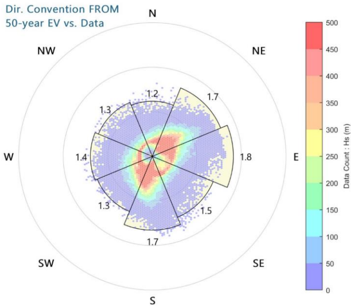
Plate 1.1.21 Wave rose of extreme wave heights at 1:50 return period for KP 115, showing the amount of wave height data per sector and in black the extreme wave height per direction sector (ABPmer, 2024b) (ABPmer, 2024b).
