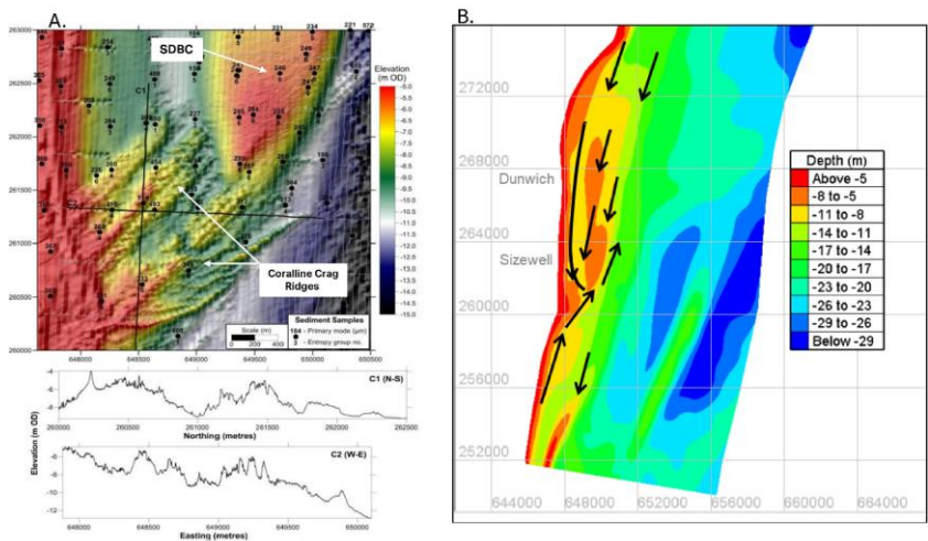
Plate 4.1.6 Bathymetry of the southern end of the trough showing ridges of Coralline Crag extending north eastwards from Thorpeness under the southern end of the SDBC. Image modified from (Mott MacDonald, 2014). B: Schematic subtidal sand transport pathways deduced from numerical modelling (BEEMS Technical Report TR357).
