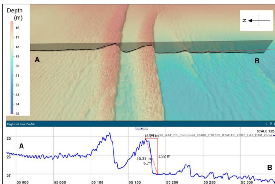
Plate 4.1.32 2 m high megaripples on the route at KP 50.5 (MMT, 2022).
