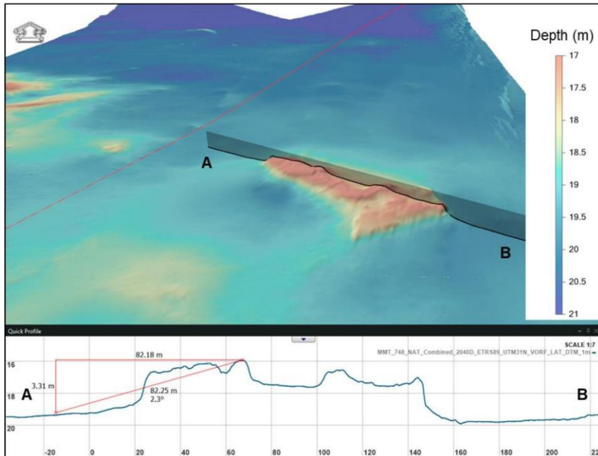
Plate 4.1.29 Outcrop at KP 8 with a height of 3.3 m above the surrounding seafloor (MMT, 2022).
