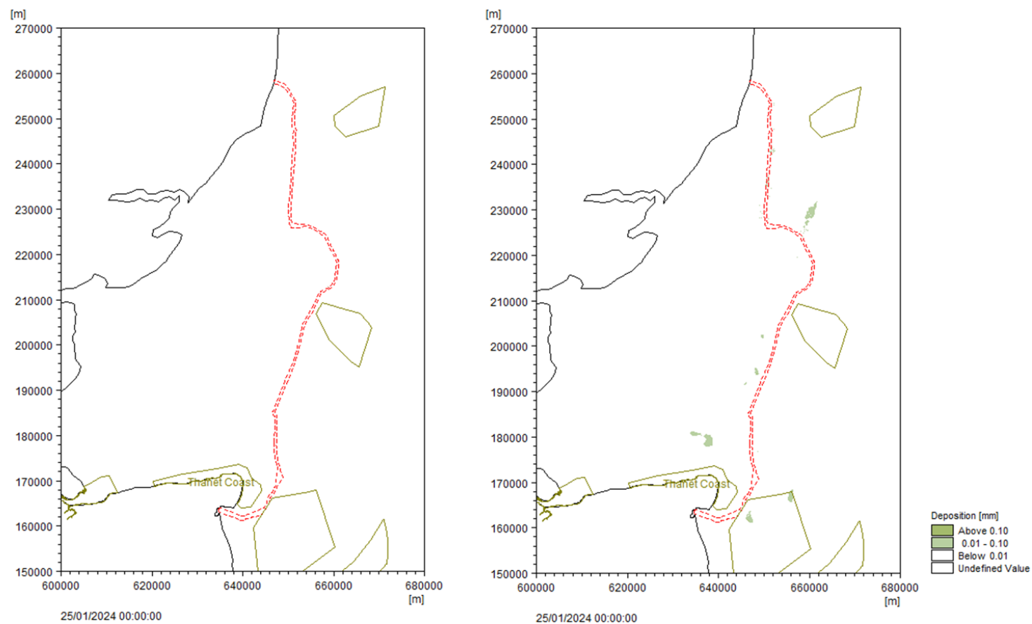
Plate 4.1.44 Depth of deposition with plough installation for mud (left) and fine sand (right) at end of 14-day period
