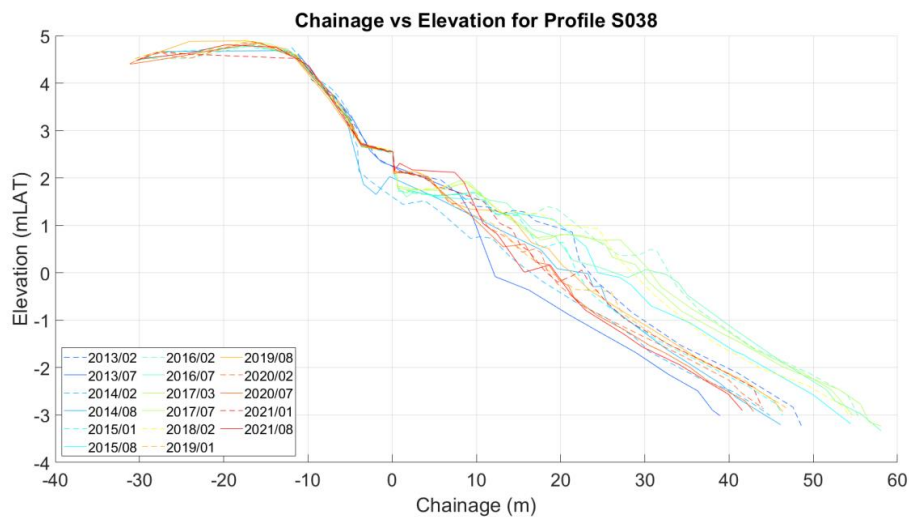
Plate 4.1.15 Profile changes 2013-2021 – Profile S038 (ABPmer, 2024a)
