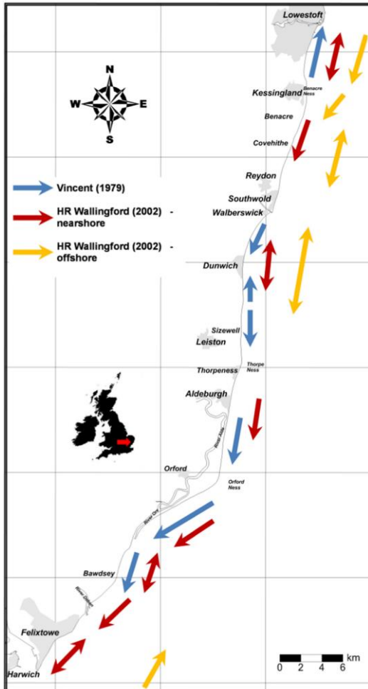
Plate 1.1.4 Potential littoral transport as estimated by (Vincent, 1979) and schematic sediment transport pathways (HR Wallingford, 2002)
