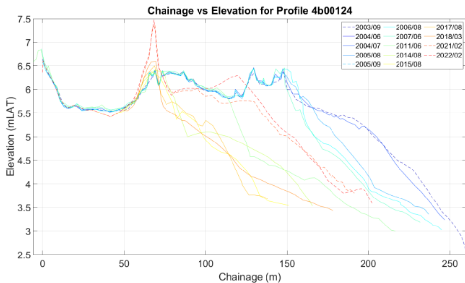
Plate 4.1.24. Profile 4b000124 elevation change (ABPmer, 2024b)
