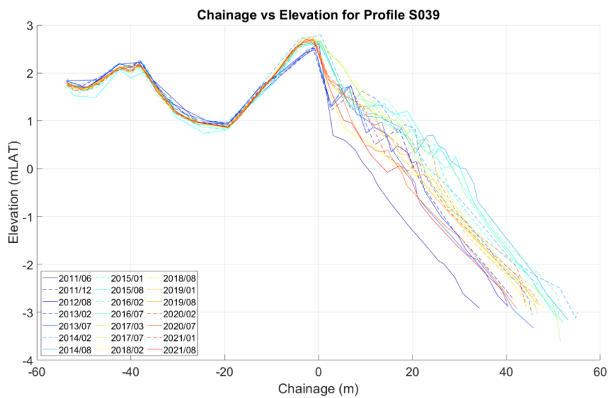
Plate 4.1.16 Profile changes 2011-2021 – Profile S039 (ABPmer, 2024a)
